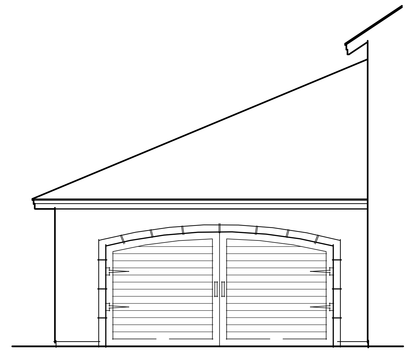
GARAGE ELEVATION
