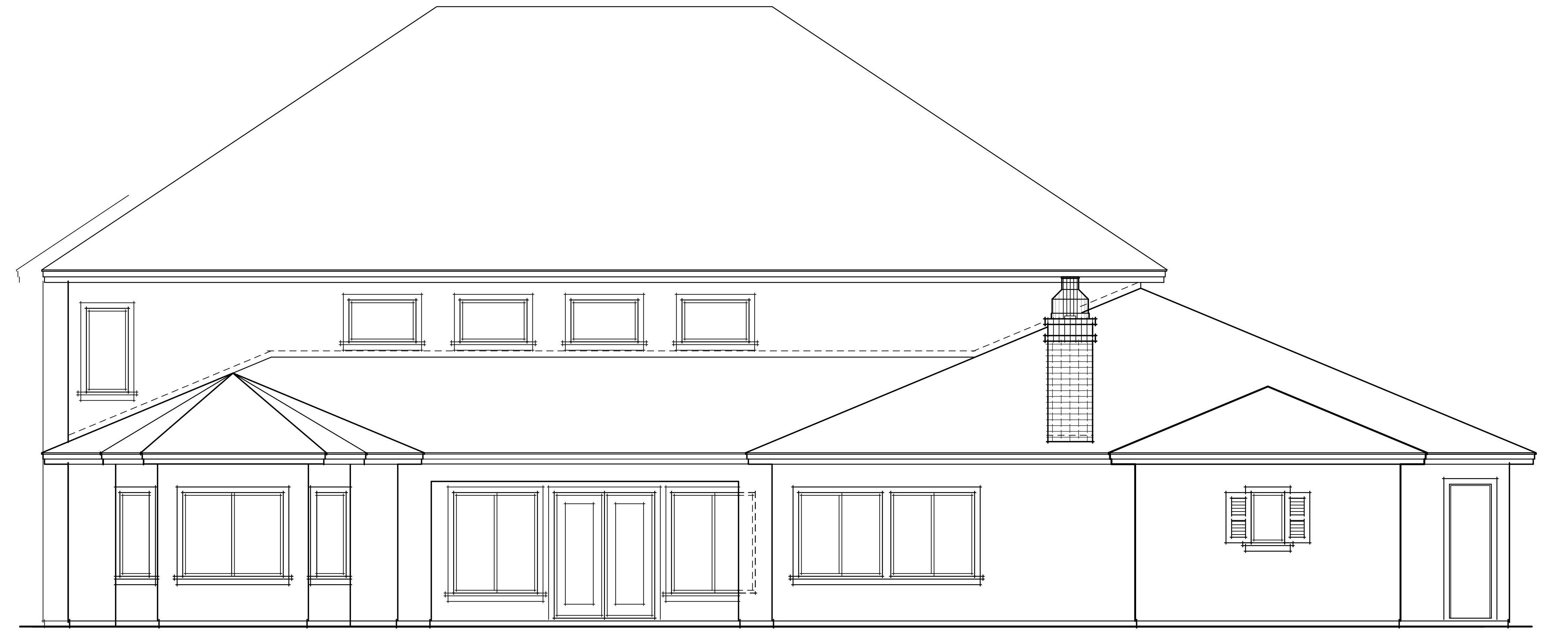
REAR ELEVATION
