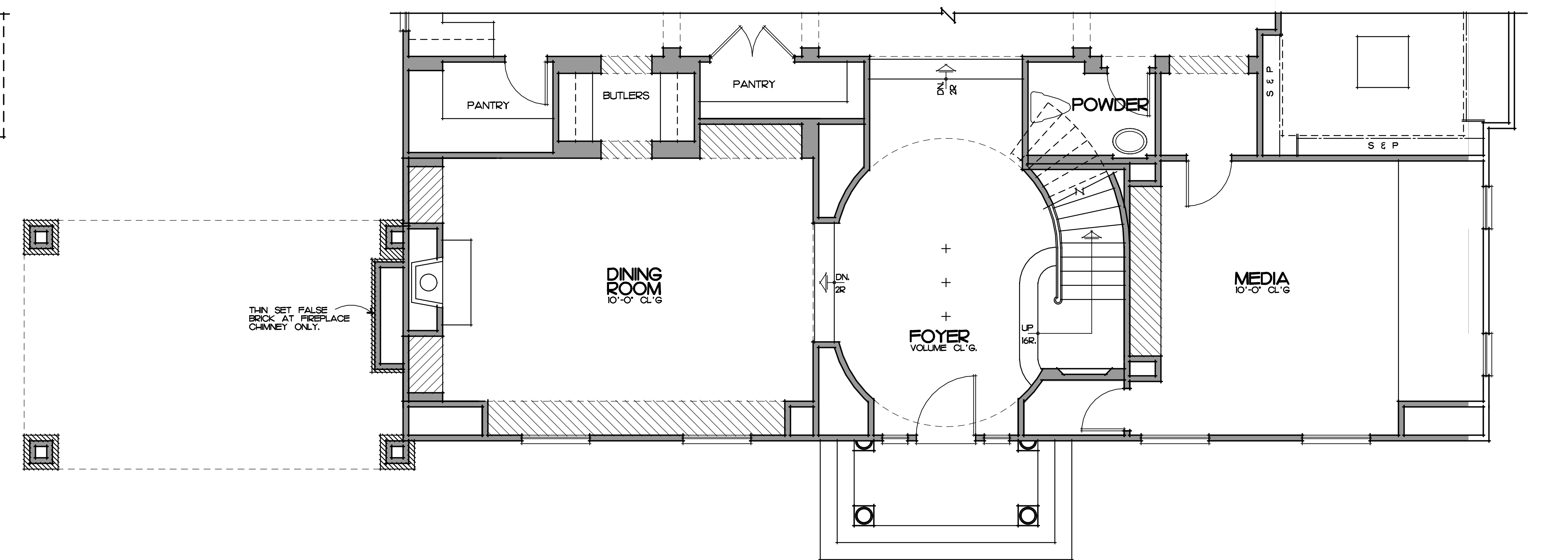
FIRST FLOOR PLAN ADDENDA
