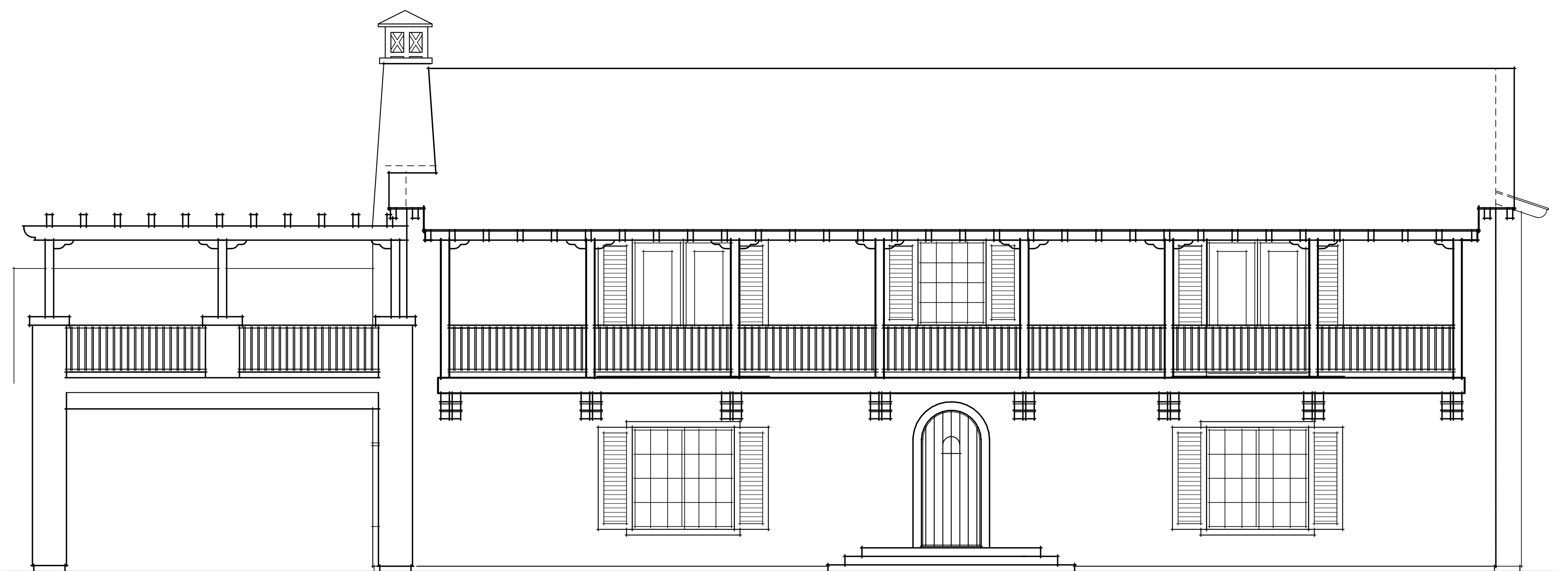
FRONT ELEVATION
