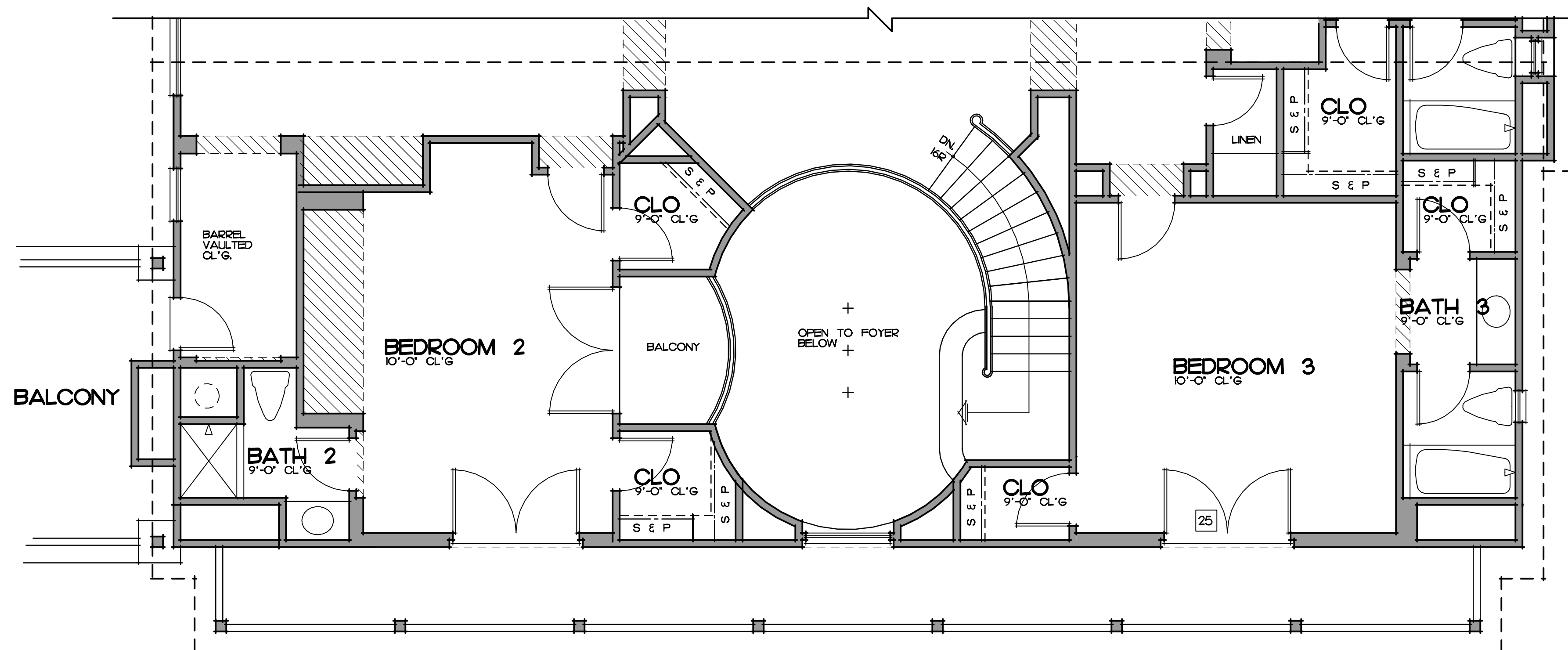
SECOND FLOOR PLAN ADDENDA
