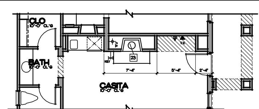
OPTIONAL FIREPLACE AT CASITA
