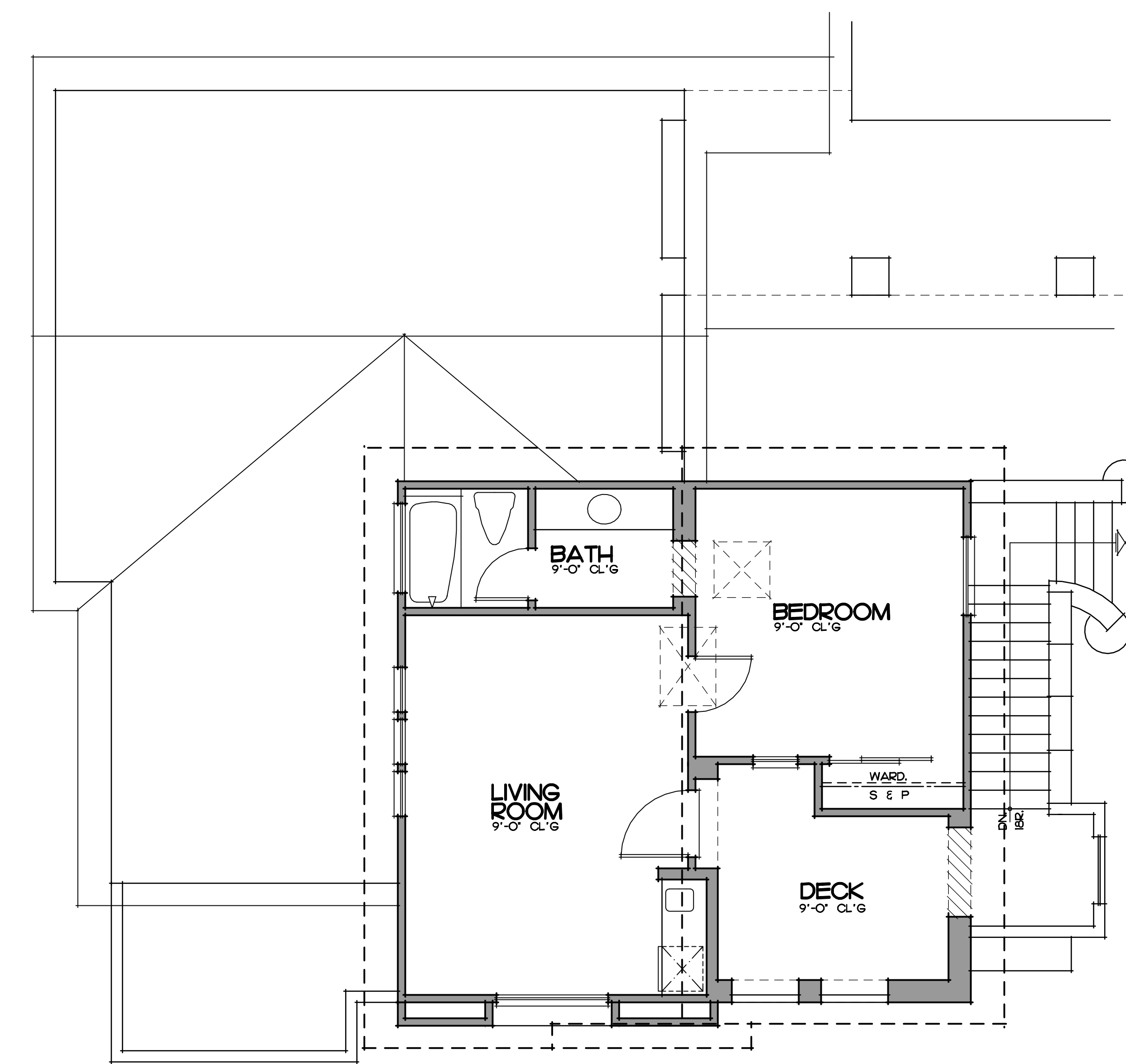
OPTIONAL CARRIAGE UNIT PLAN 'A' SCALE: 1/4" = 1'-0" ONE BEDROOM SUITE
