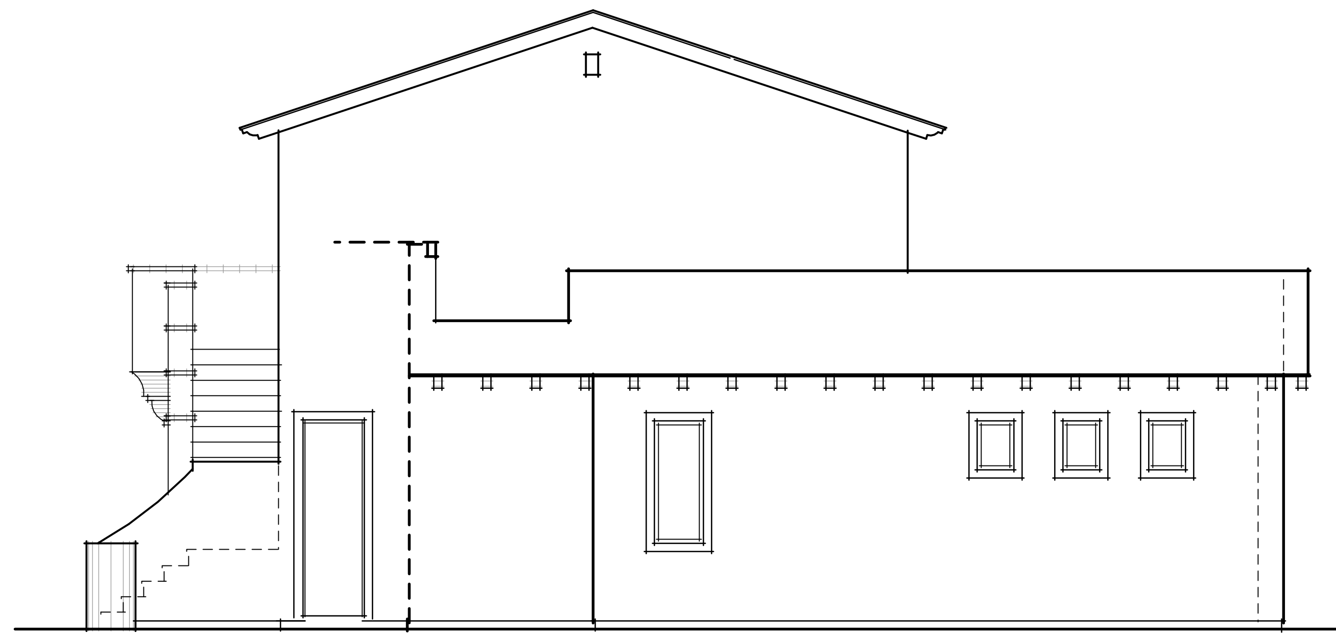
CASITA/ CARRIAGE UNIT REAR ELEV 'A'
