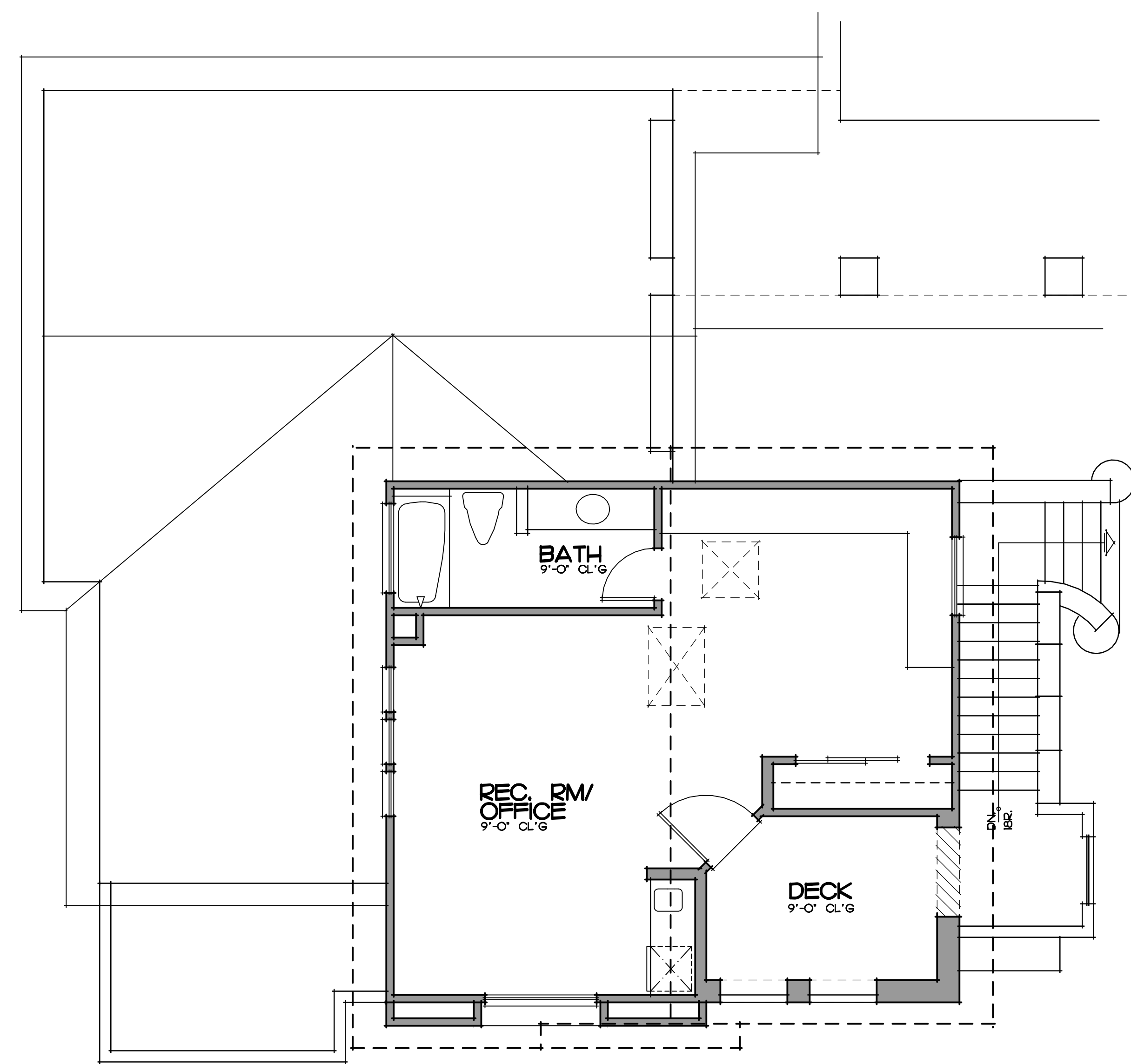
OPTIONAL CARRIAGE UNIT PLAN 'A' SCALE: 1/4" = 1'-0" REC. ROOM / OFFICE
