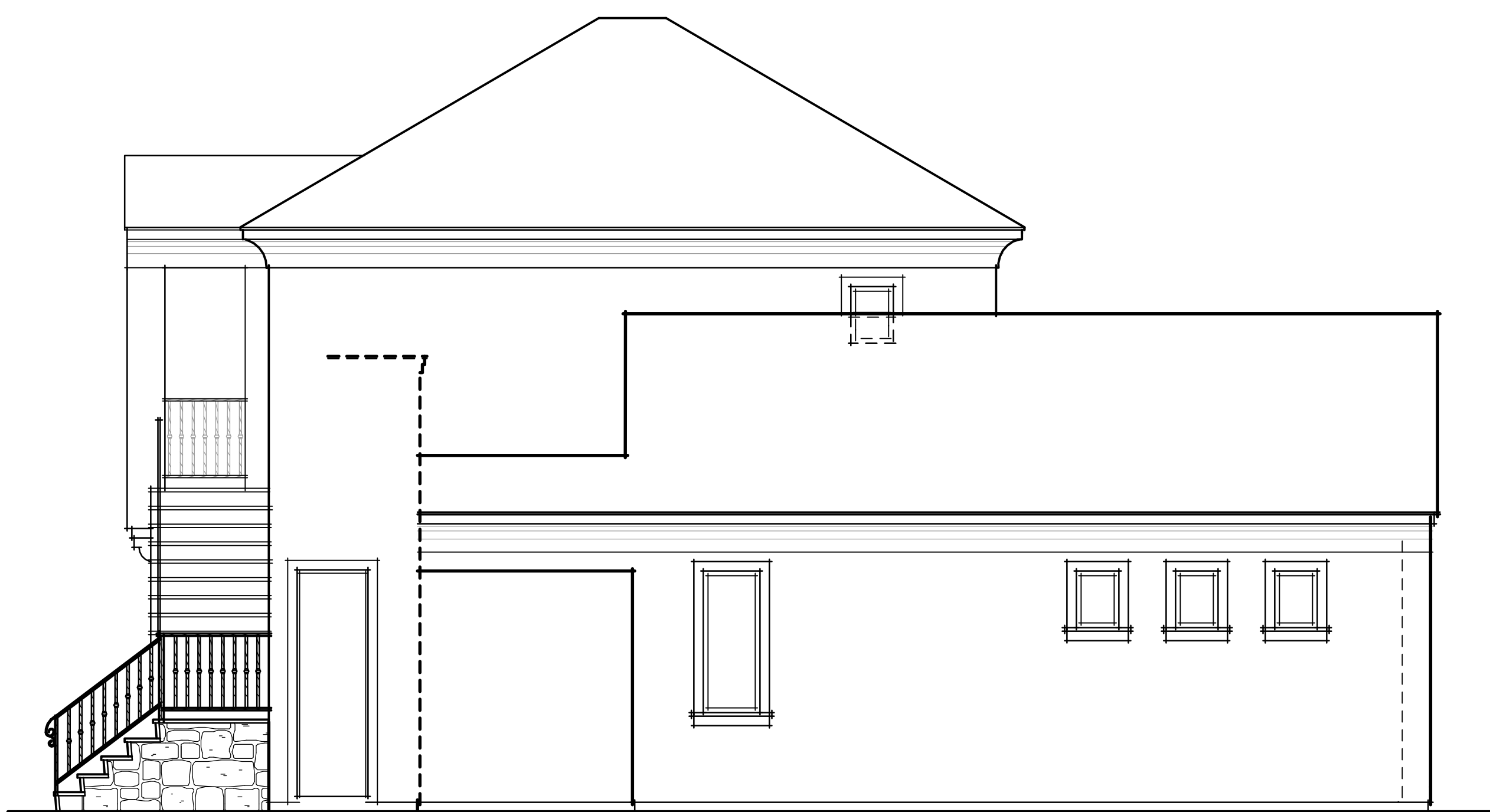
CASITA/ CARRIAGE UNIT REAR ELEV 'B'
