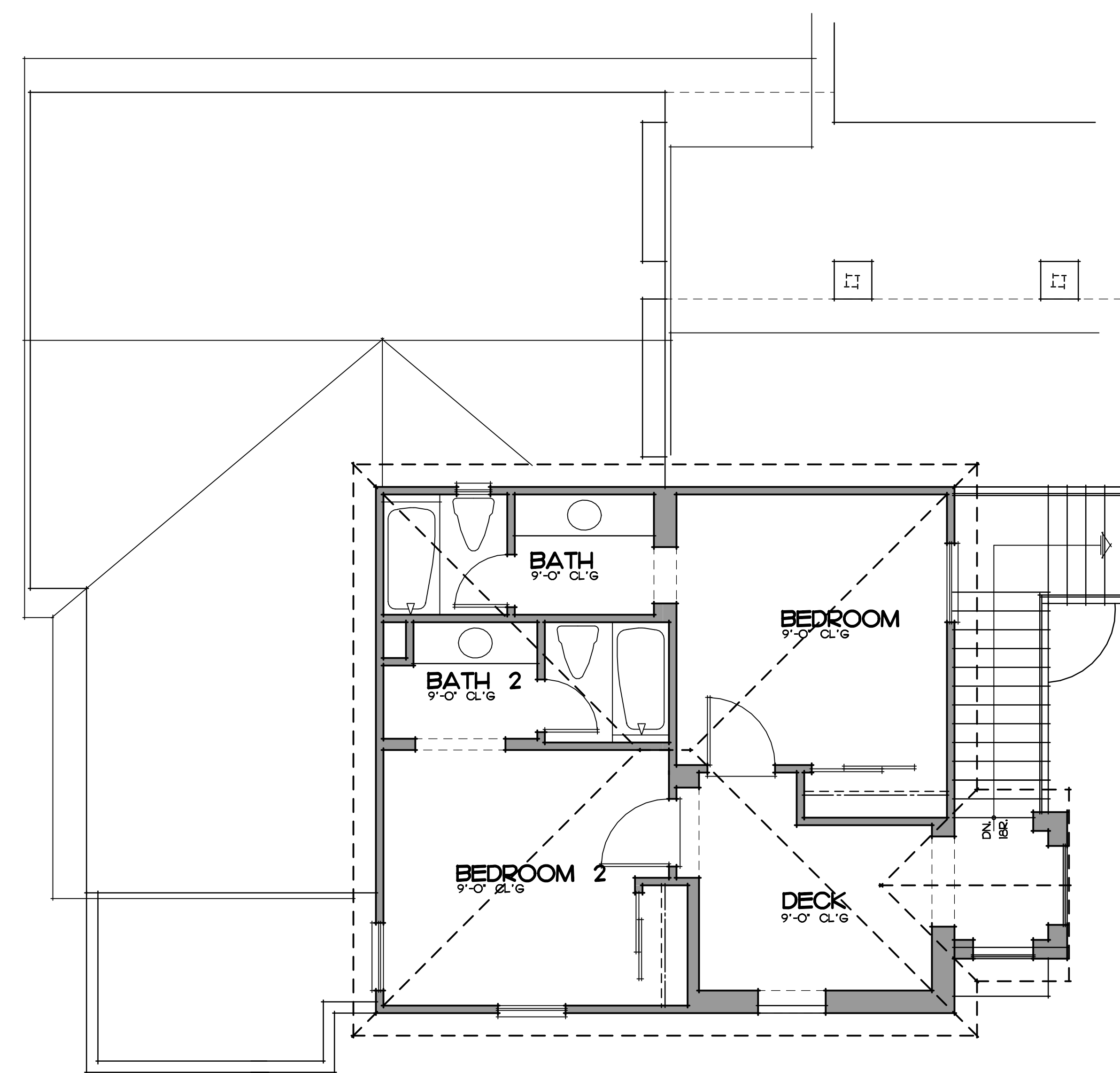
OPTIONAL CARRIAGE UNIT PLAN 'B' SCALE: 1/4" = 1'-0" TWO BEDROOM SUITE
