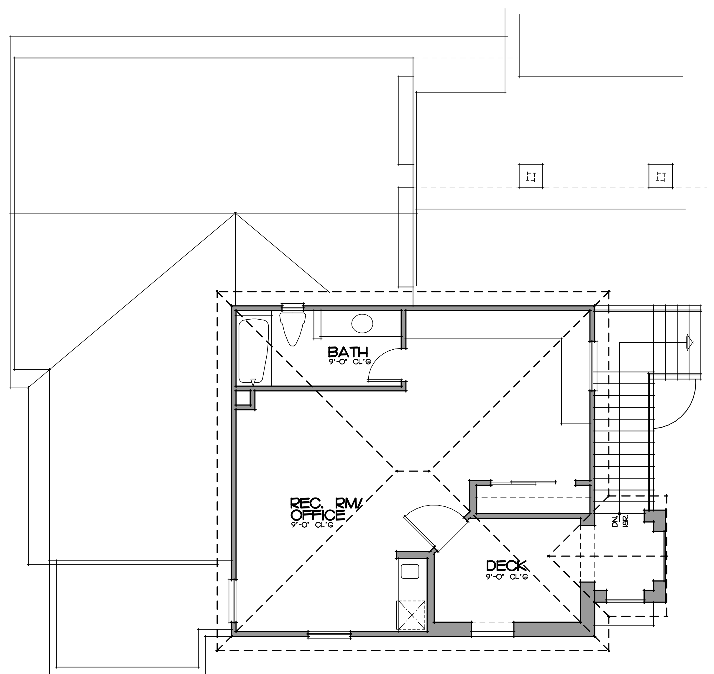
OPTIONAL CARRIAGE UNIT PLAN 'B' SCALE: 1/4" = 1'-0" REC. ROOM / OFFICE
