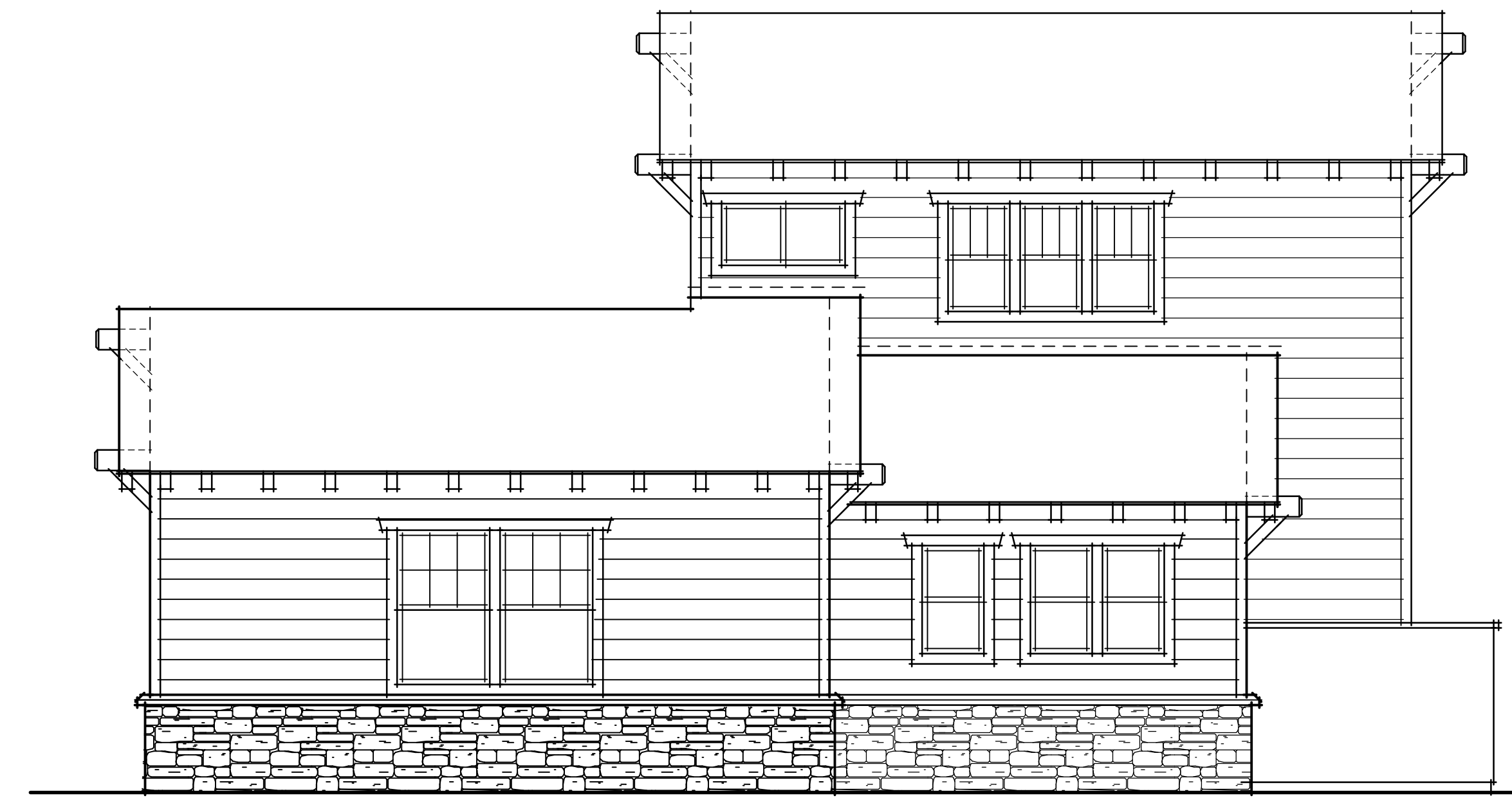
CASITA/ CARRIAGE UNIT LEFT ELEV 'C'
