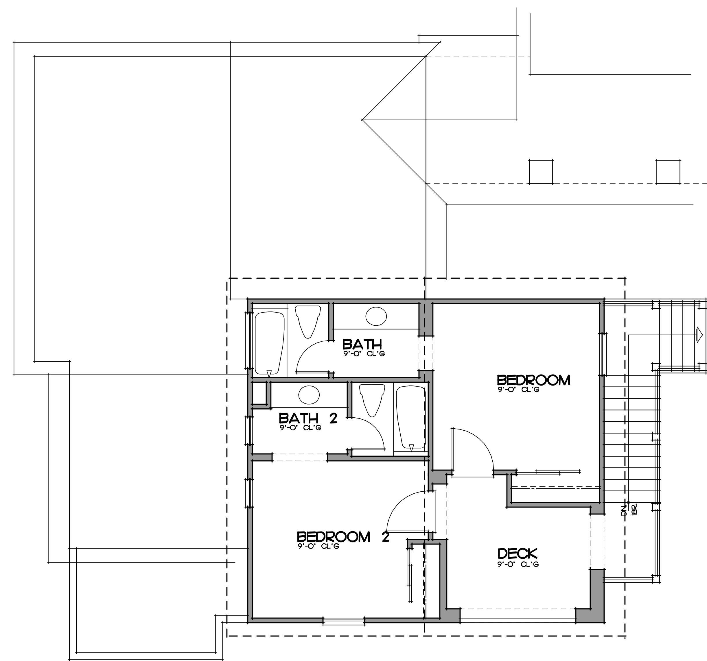
OPTIONAL CARRIAGE UNIT PLAN 'C' SCALE: 1/4" = 1'-0" TWO BEDROOM SUITE
