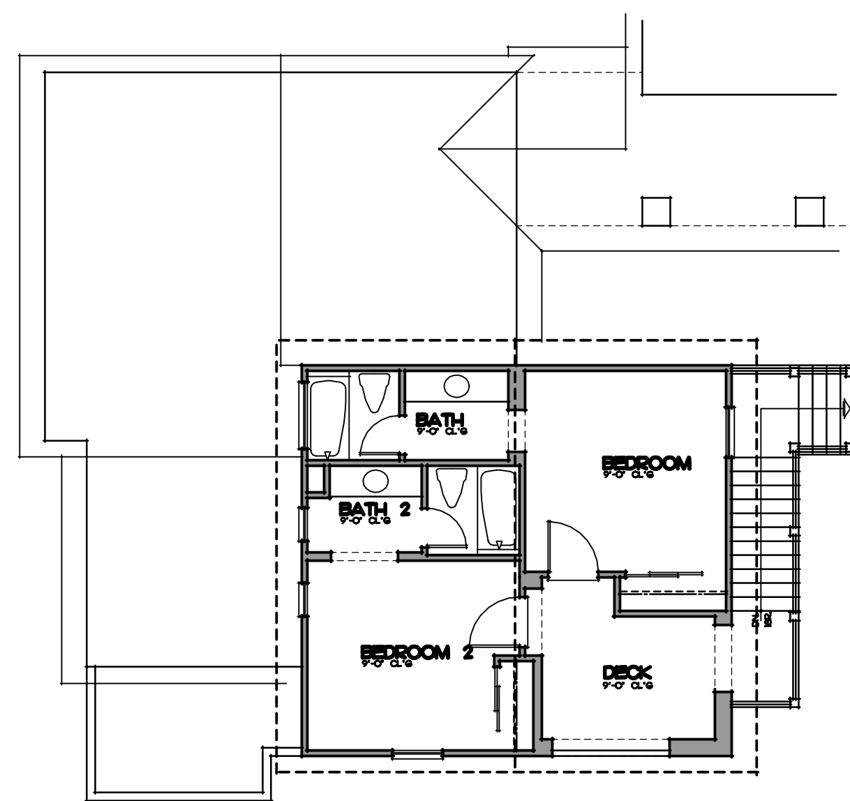
OPTIONAL CARRIAGE UNIT PLAN 'C' SCALE: 1/8" = 1'-0" TWO BEDROOM SUITE
