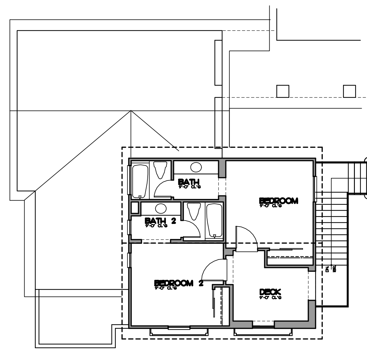
OPTIONAL CARRIAGE UNIT PLAN 'D' SCALE: 1/4" = 1'-0" TWO BEDROOM SUITE
