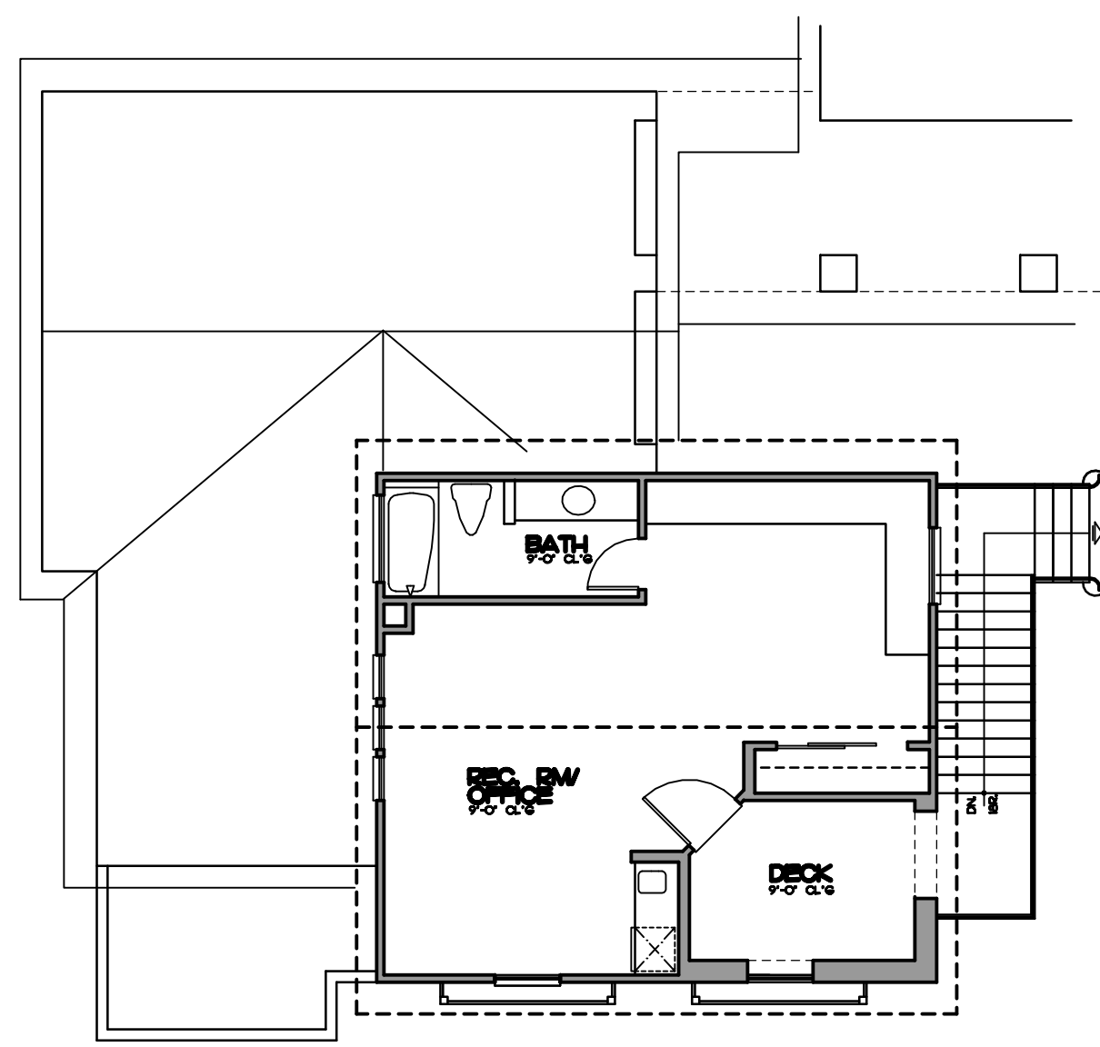
OPTIONAL CARRIAGE UNIT PLAN 'D' SCALE: 1/4" = 1'-0" REC. ROOM / OFFICE
