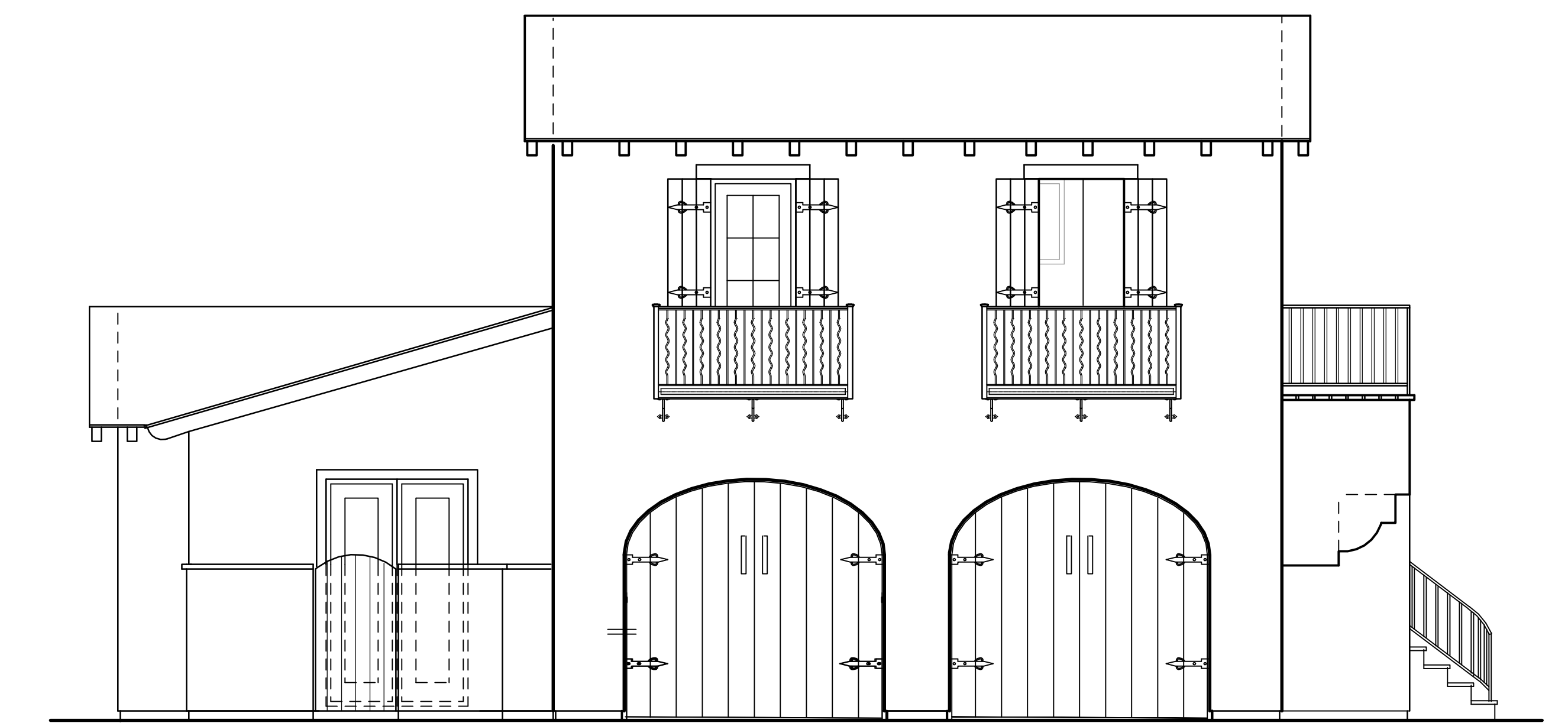
CASITA/ CARRIAGE UNIT FRONT ELEV 'D'
