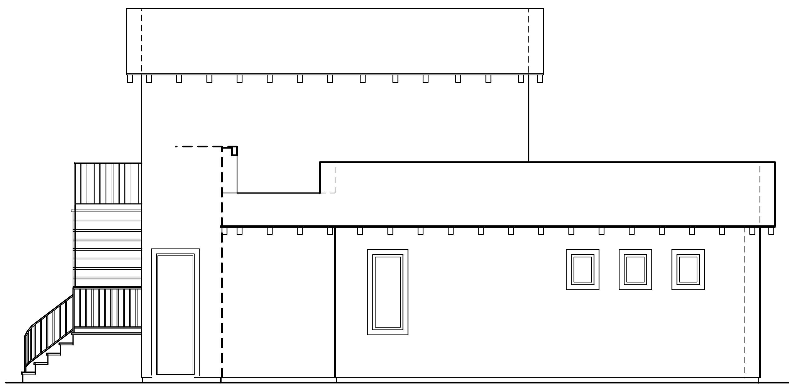
CASITA/ CARRIAGE UNIT REAR ELEV 'D'
