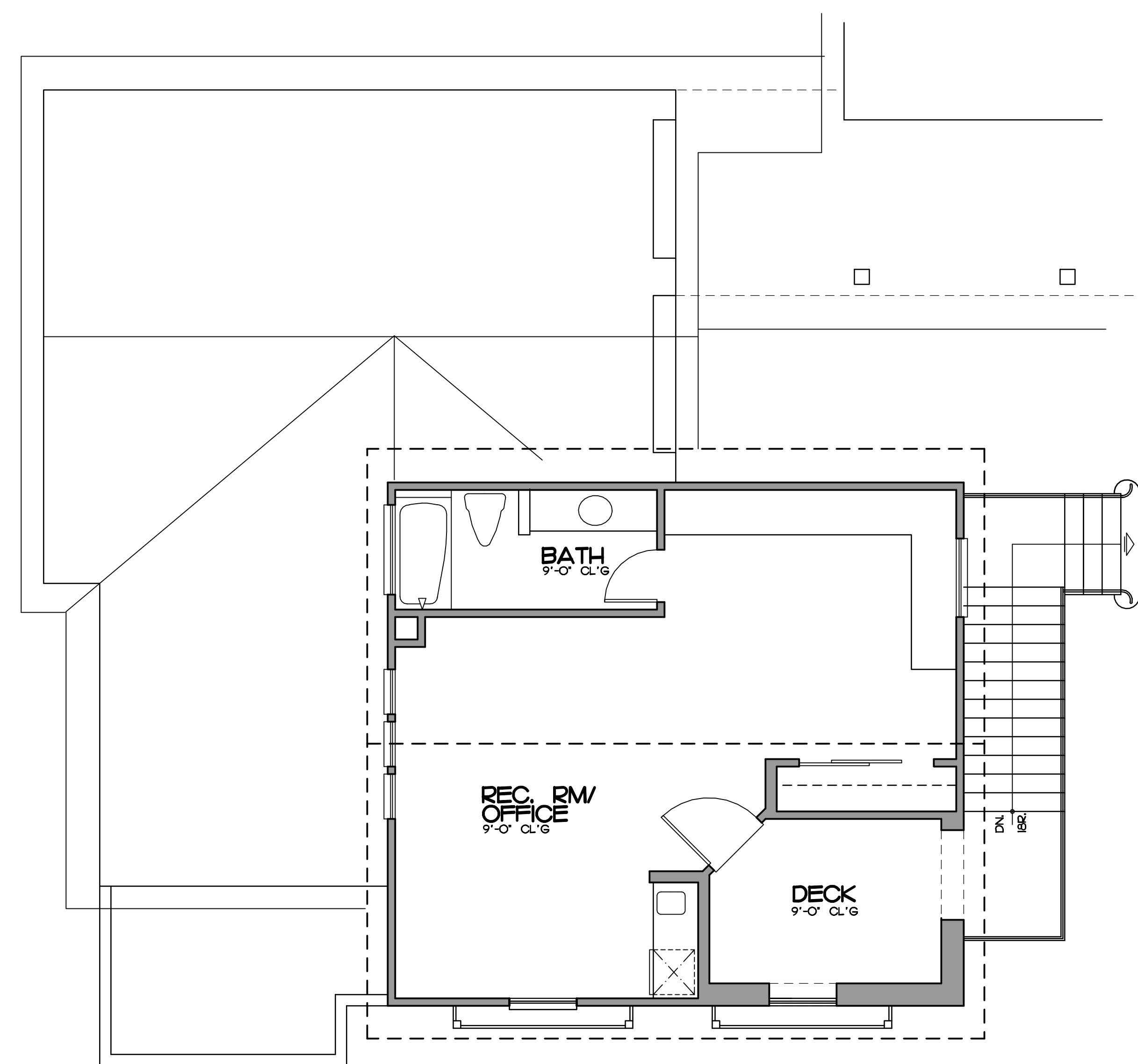
OPTIONAL CARRIAGE UNIT PLAN 'D' REC. ROOM / OFFICE
