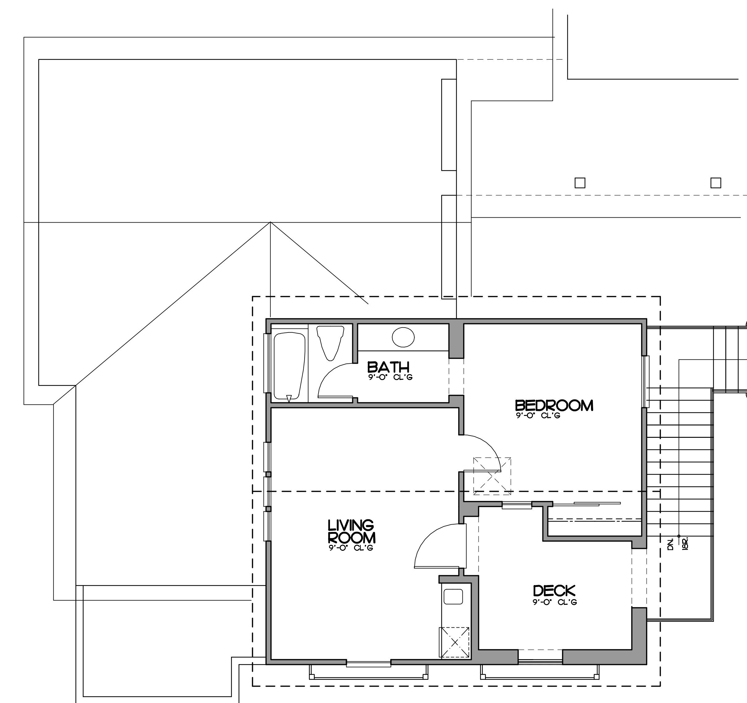
OPTIONAL CARRIAGE UNIT PLAN 'D' ONE BEDROOM SUITE
