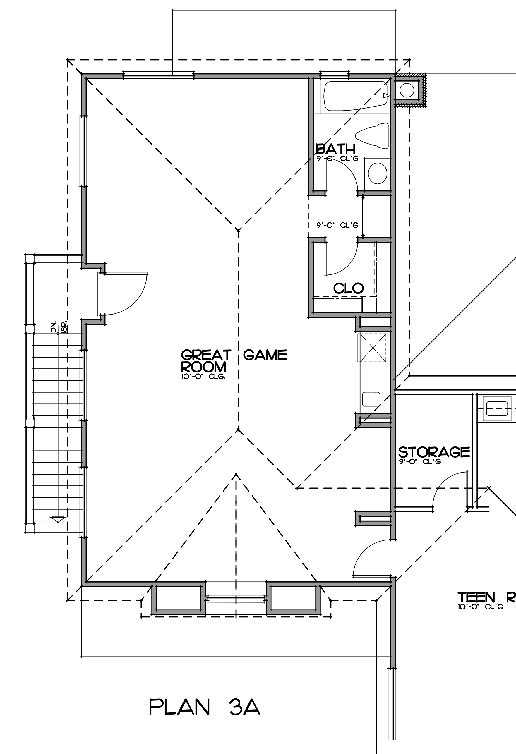
OPTIONAL GREAT GAME ROOM/ BATH CARRIAGE UNIT SCALE: 1/4" = 1'-0" +795 SQ. FT.
