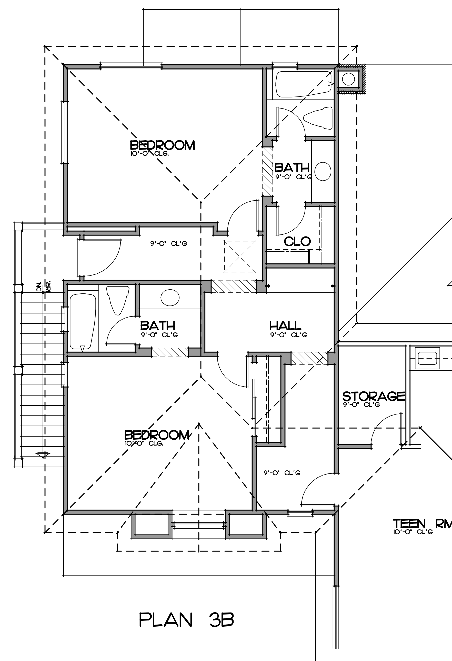
OPTIONAL 2-BEDROOM/ 2-BATH CARRIAGE UNIT SCALE: 1/4" = 1'-0" +795 SQ. FT.
