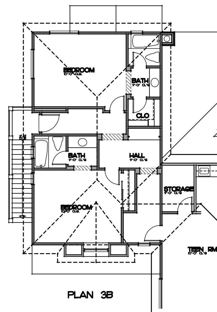
PLAN 3B OPTIONAL 2-BEDROOM / 2-BATH CARRIAGE UNIT 795 SQ. FT. SCALE: 1/4" = 1'-0"
