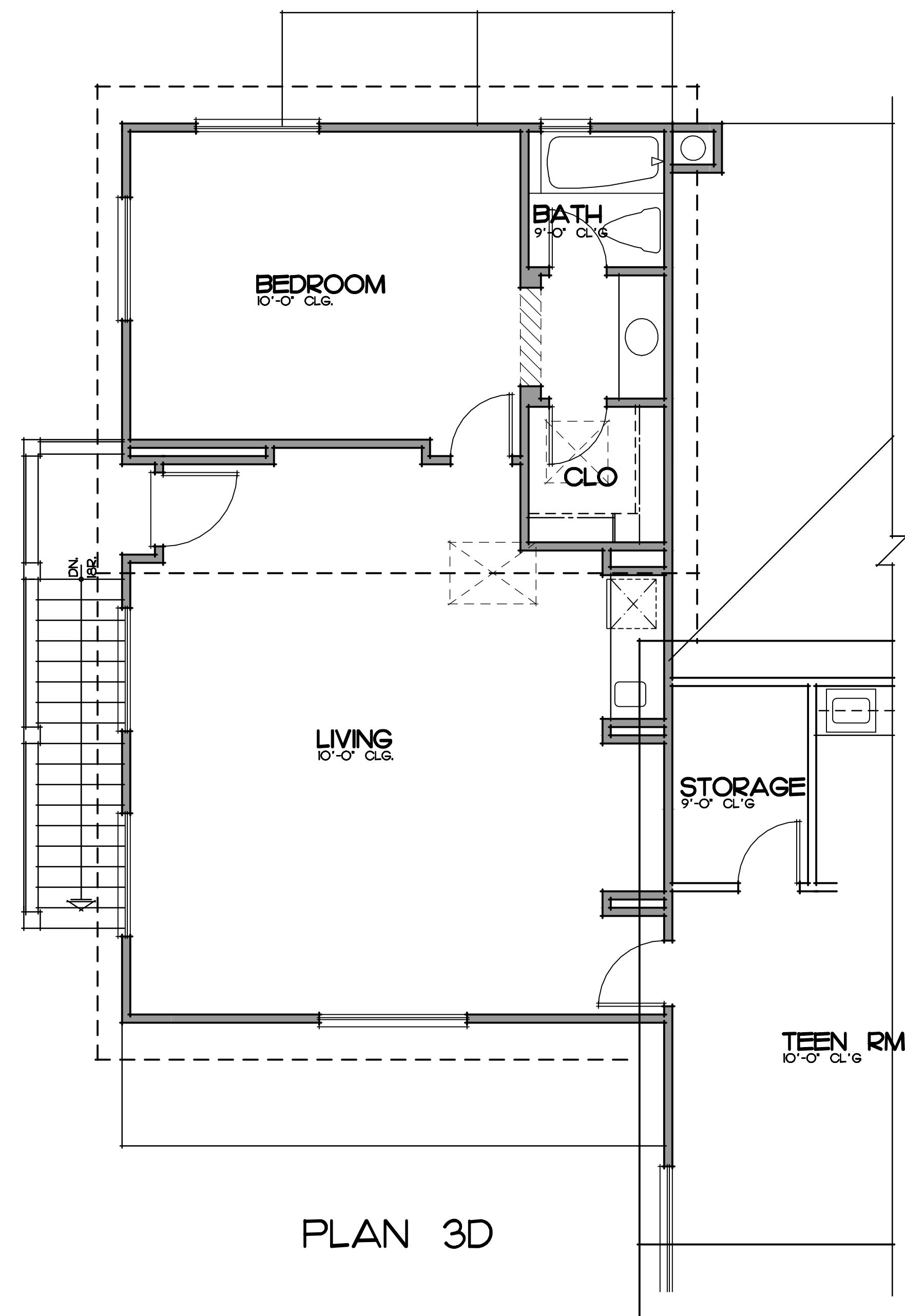
OPTIONAL BEDROOM / BATH / LIVING RM SCALE: 1/4" = 1'-0" CARRIAGE UNIT +795 SQ. FT.
