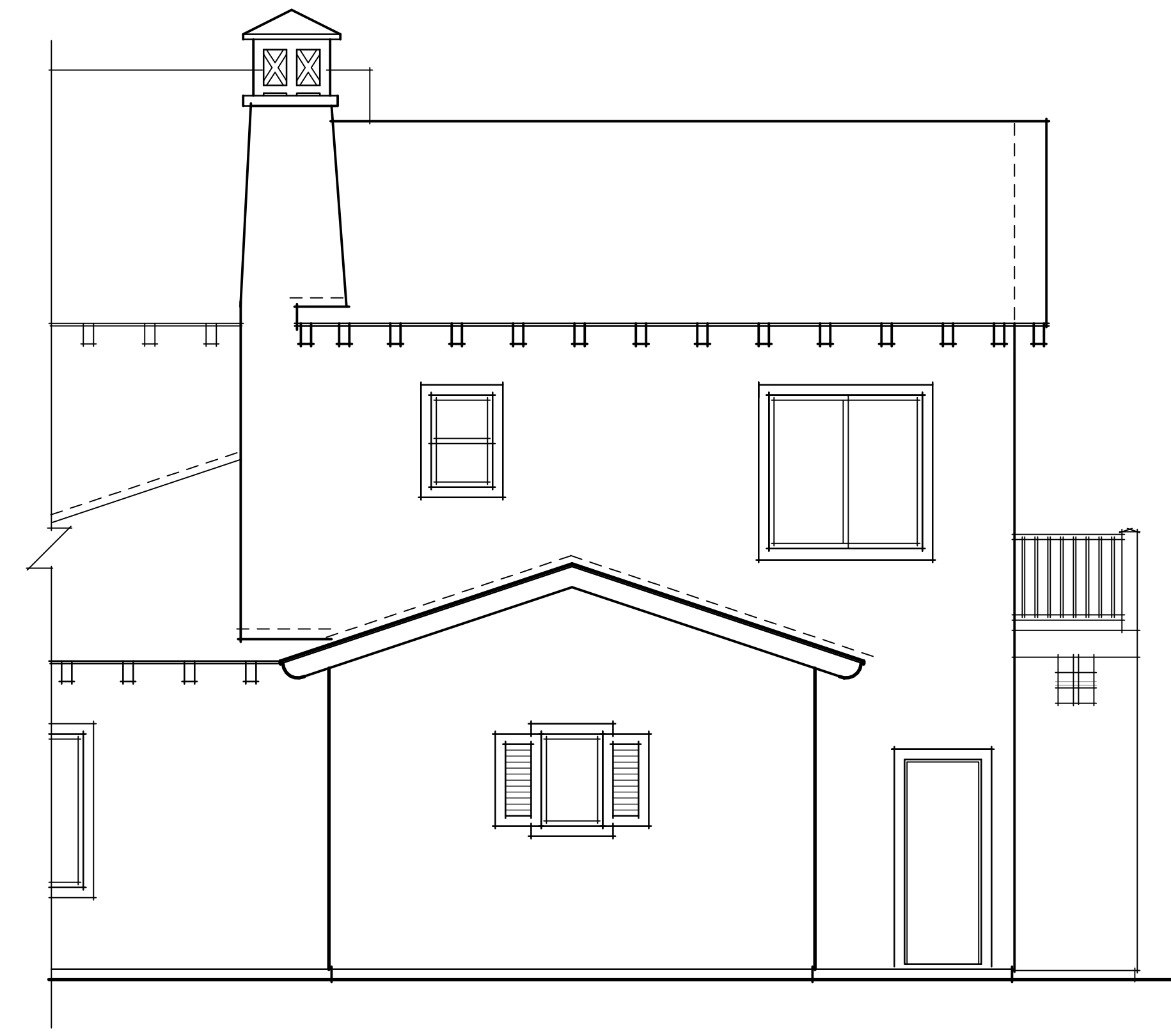
OPTIONAL REAR ELEV 'D' CARRIAGE UNIT
