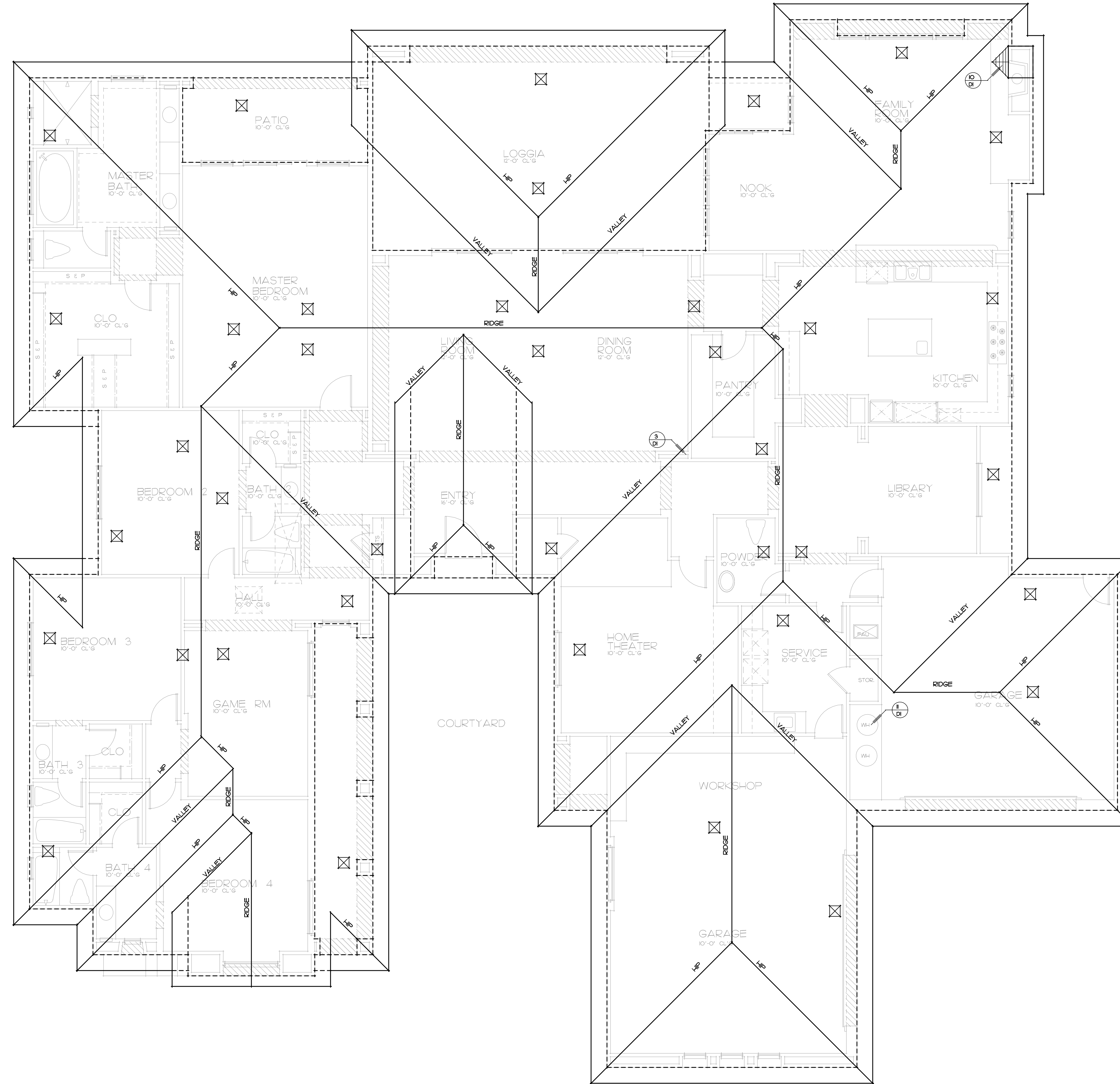
ROOF PLAN
