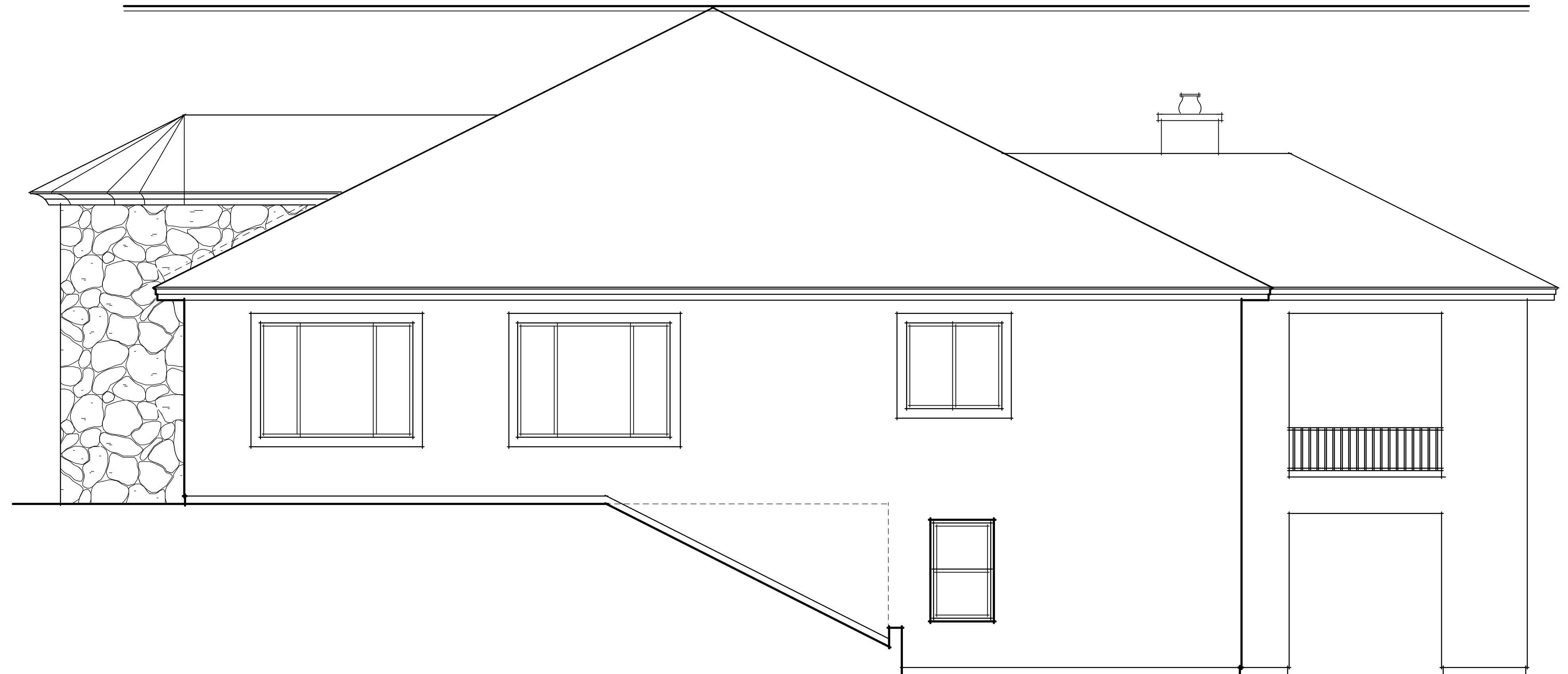
LEFT ELEVATION
